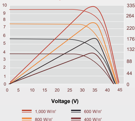
I-V Curves at different irradiances (335W)
